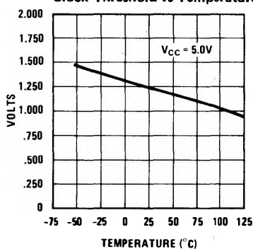
Clock Threshold vs Temperature
