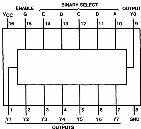
Order Number DM74184N or DM74185AN See NS Package Number N16E
