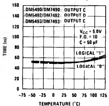
Transition Time to Outputs C &amp; D
