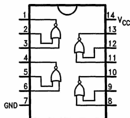
Dual-In-Line Package
