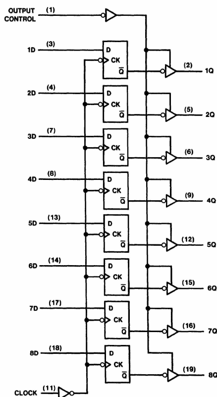
Positive-Edge-Triggered Flip-Flops
