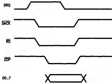
FIGURE 4.8.1. Non-Block DMA Timing
