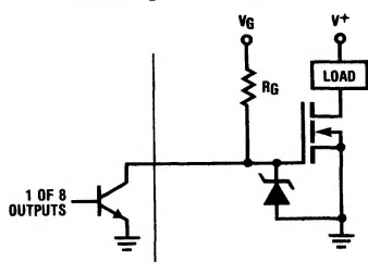
VMOS High Current Driver
