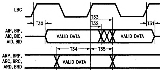
FIGURE 7-7. PHY Port Interface Timing
