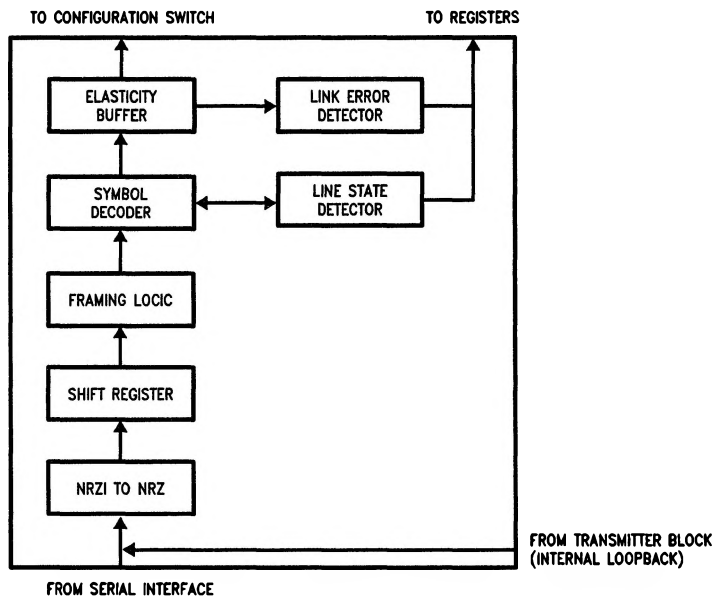
FIGURE 3-1. Receiver Block Diagram
