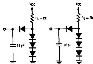
Load Circuit 1
