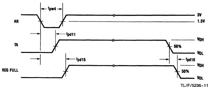
FIGURE 10. Auto-Response
