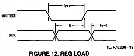
FIGURE 12. REG LOAD
