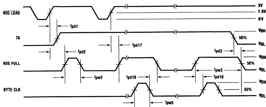
FIGURE 7. Two-Byte Transfer
