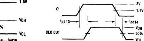
FIGURE 11. Clock Pulse
