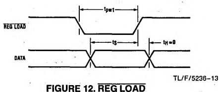
FIGURE 12. REG LOAD
