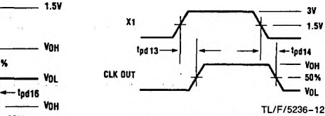
FIGURE 11. Clock Pulse
