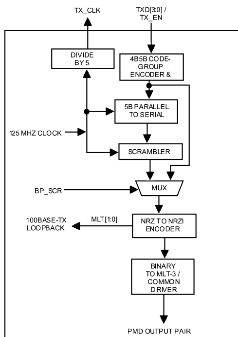
Figure 4-3. 100BASE-TX Transmit Block Diagram
