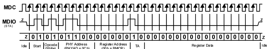
Figure 4-2. Typical MDC/MDIO Write Operation
