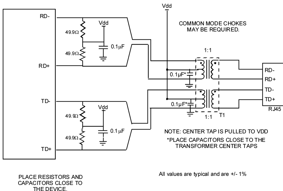
Figure 4-8. 10/100 Mb/s Twisted Pair Interface
