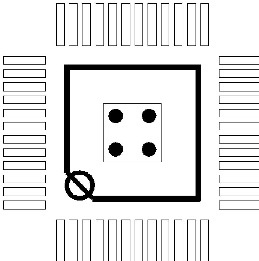
Figure 4-11. Top View, Thermal Vias for GNDPAD, Pin 49
