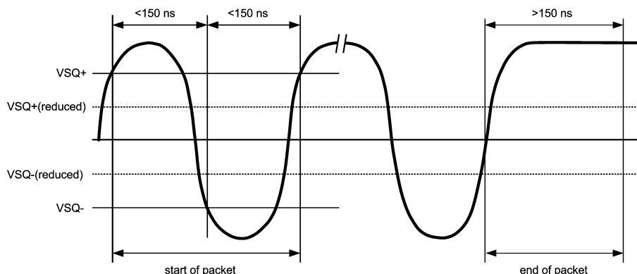
Figure 4-7. 10BASE-T Twisted Pair Smart Squelch Operation
