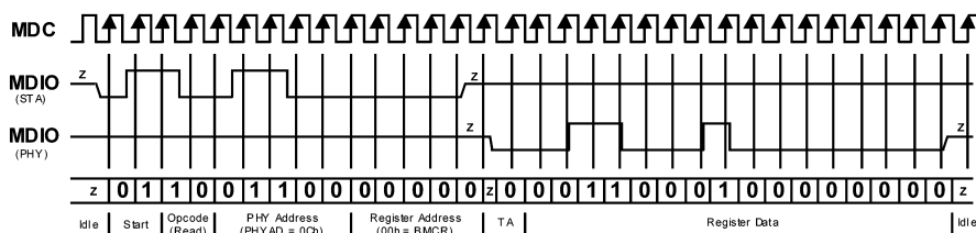
Figure 4-1. Typical MDC/MDIO Read Operation
