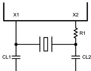
Figure 4-9. Crystal Oscillator Circuit
