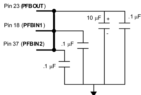
Figure 4-10. Power Feedback Connection
