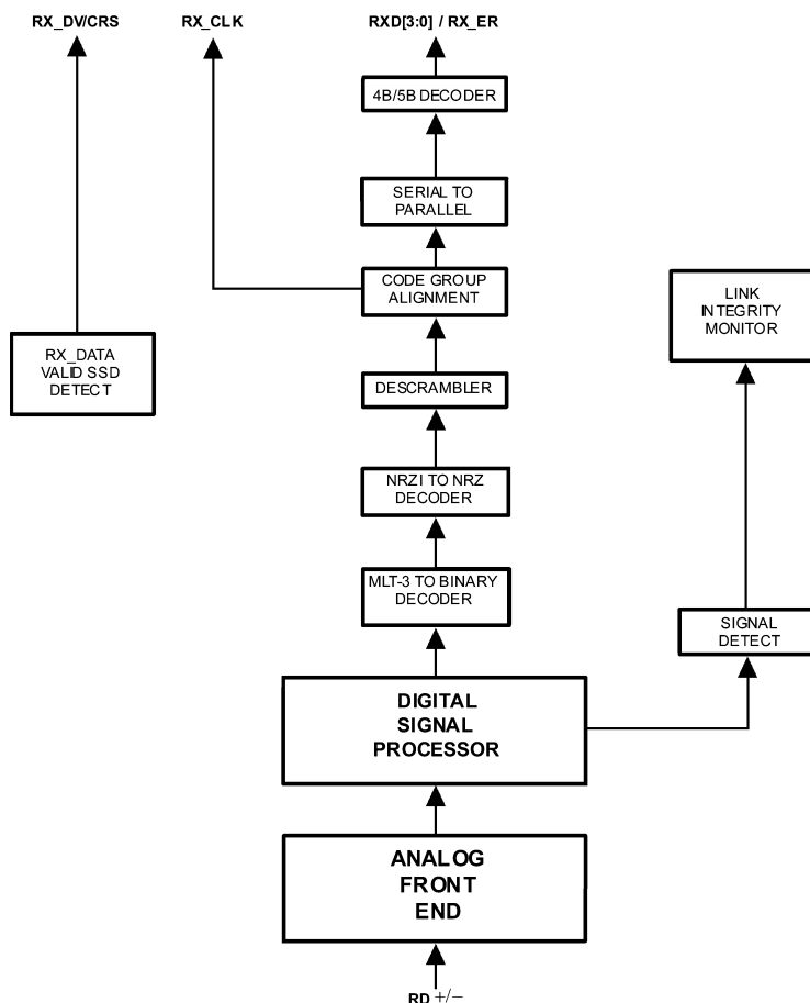
Figure 4-4. 100BASE-TX Receive Block Diagram
