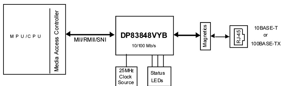
Typical Application
