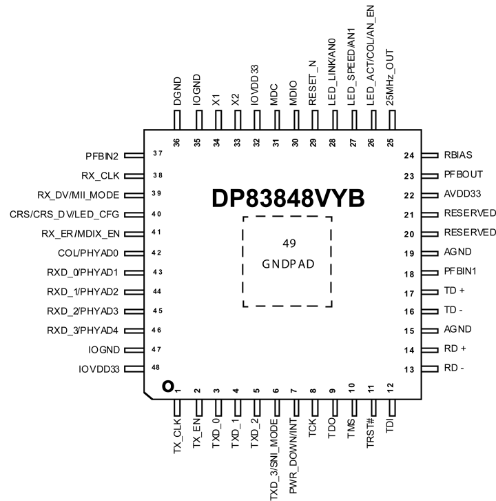
Figure 2-1. Top View Package Number PTB0048A
