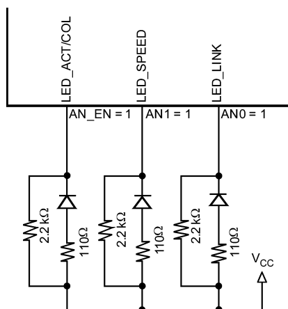
Figure 3-2. AN Strapping and LED Loading Example
