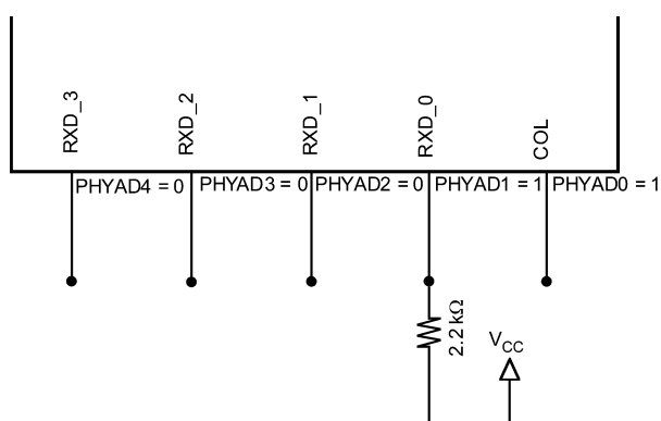
Figure 3-1. PHYAD Strapping Example
