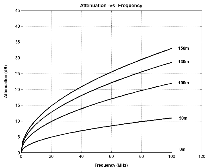
Figure 4-5. EIA/TIA Attenuation vs. Frequency for 0, 50, 100, 130 & 150 Meters of CAT 5 Cable
