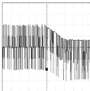
Figure 4-6. 100BASE-TX BLW Event
