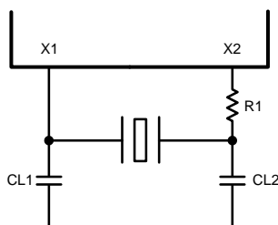
Figure 7-3. Crystal Oscillator Circuit
