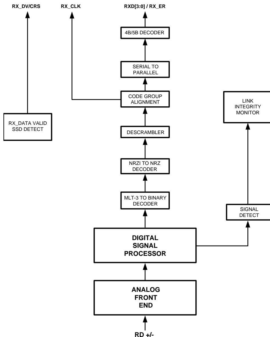
Figure 6-2. 100BASE-TX Receive Block Diagram
