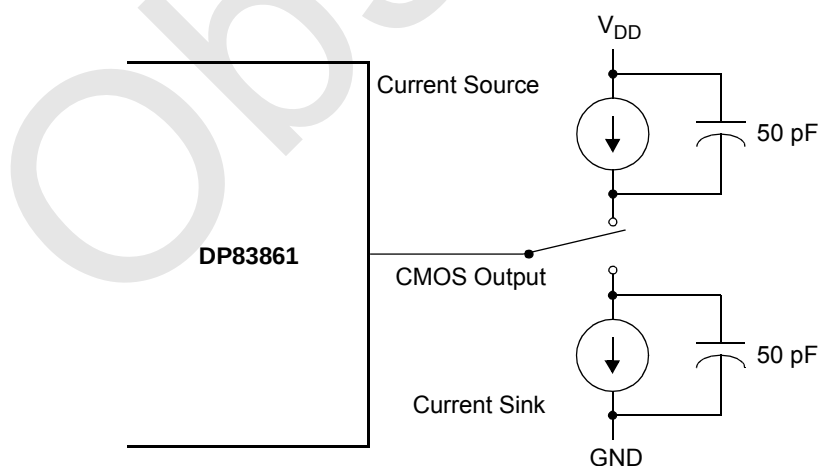
Figure 17. CMOS Output Test Load
