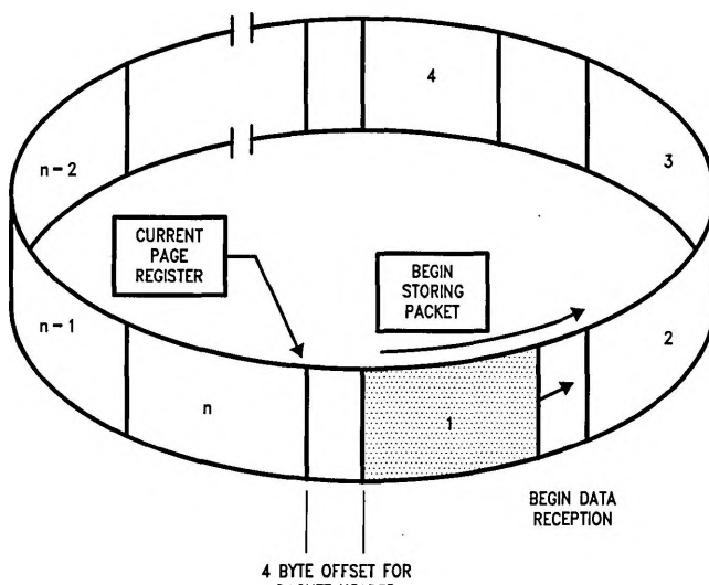
Received Packet Enters the Buffer Pages
