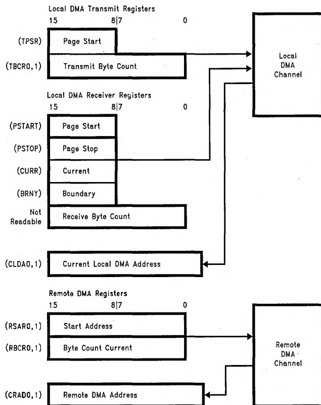
FIGURE 24. DMA Registers
