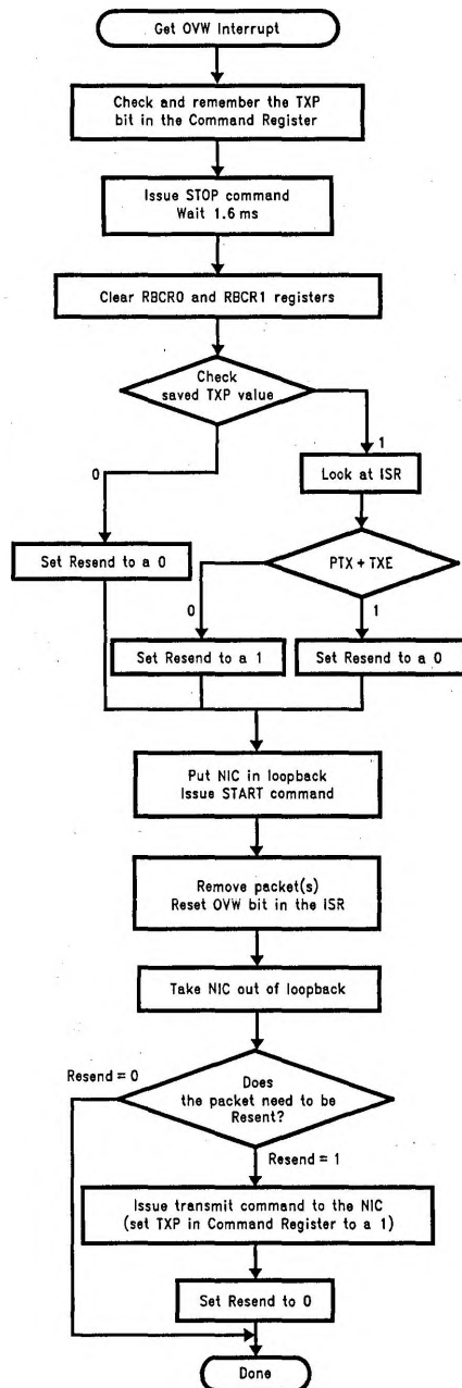
FIGURE 32. Overflow Routine
