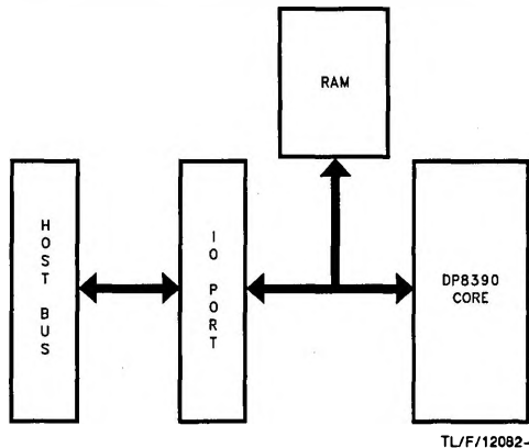
FIGURE 2. I/O Port
