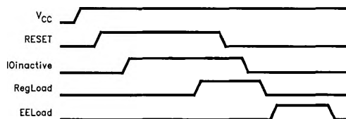
FIGURE 6. RESET Operation
