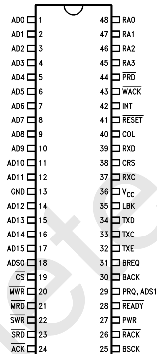
Dual-In-Line Package
