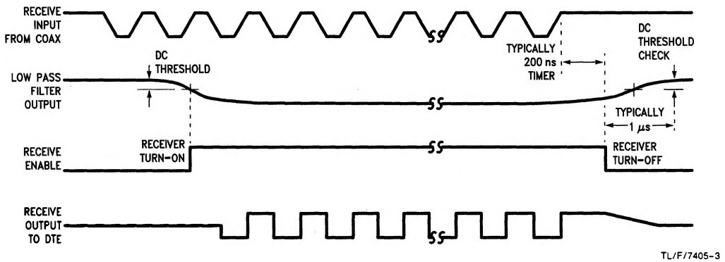
FIGURE 2. Receiver Timing
