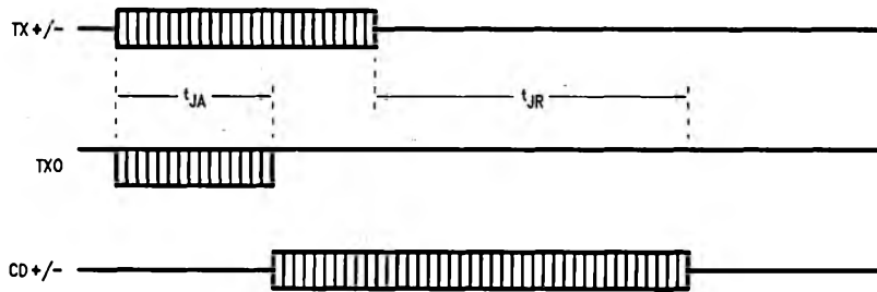
FIGURE 12. Jabber Timing
