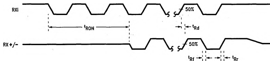
FIGURE 8. Receiver Timing
