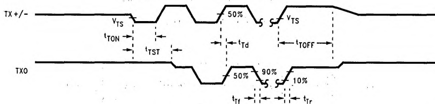
FIGURE 9. Transmitter Timing
