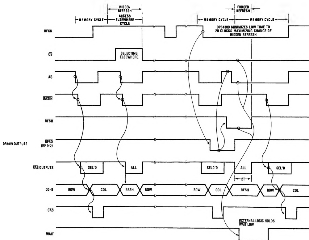
FIGURE 9. DP8419 Auto Refresh, Access with \overline{\text{WAIT}} States
