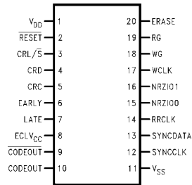
FIGURE 2. DP84902 Pinout
