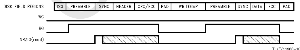
FIGURE 13. Hard Sector Read Mode Waveforms
