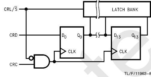
FIGURE 11. CTRL Register Block Diagram
