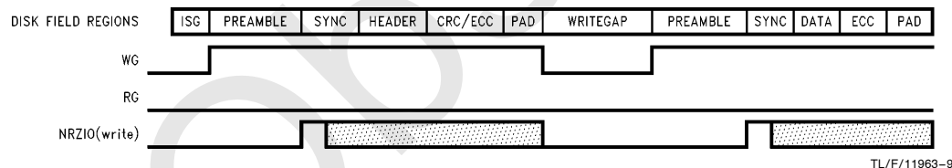
FIGURE 12. Hard Sector Write Mode Waveforms
