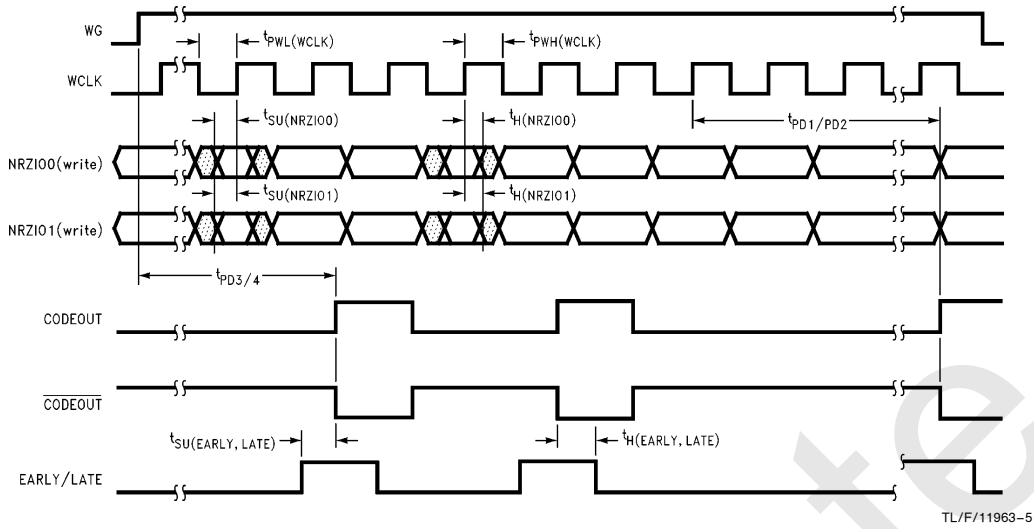
FIGURE 5. Write Timing Diagram
