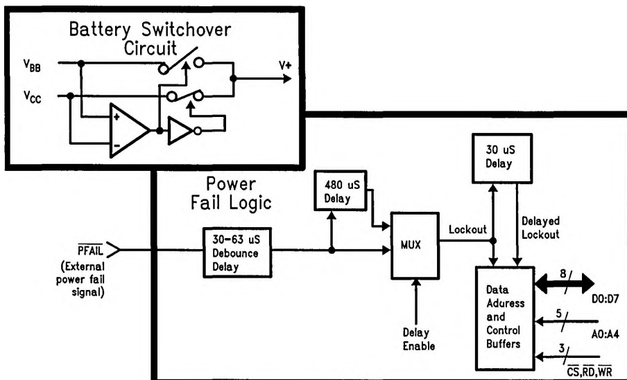
FIGURE 6. System-Battery Swover (Upper Left), Power Fail and Lock-Out Circuits (Lower Right)
