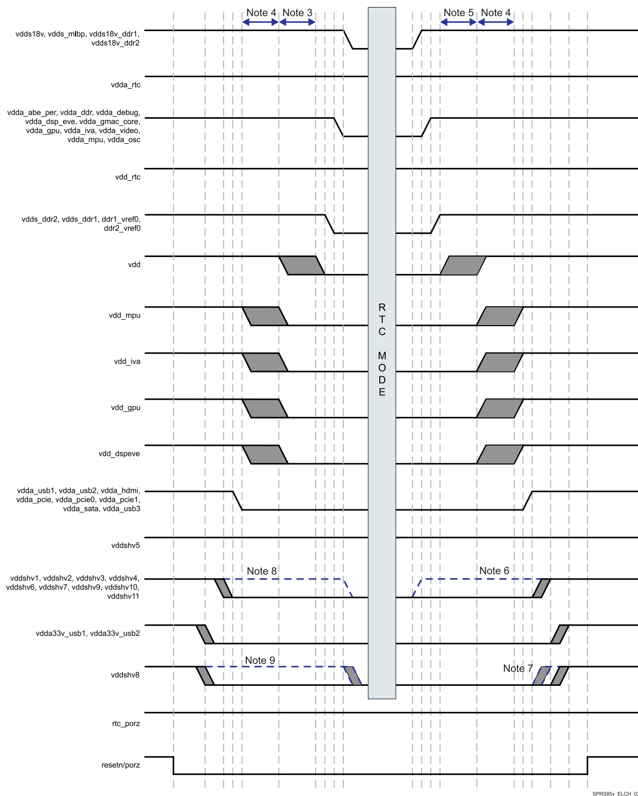
Figure 5-3. RTC Mode Sequencing
