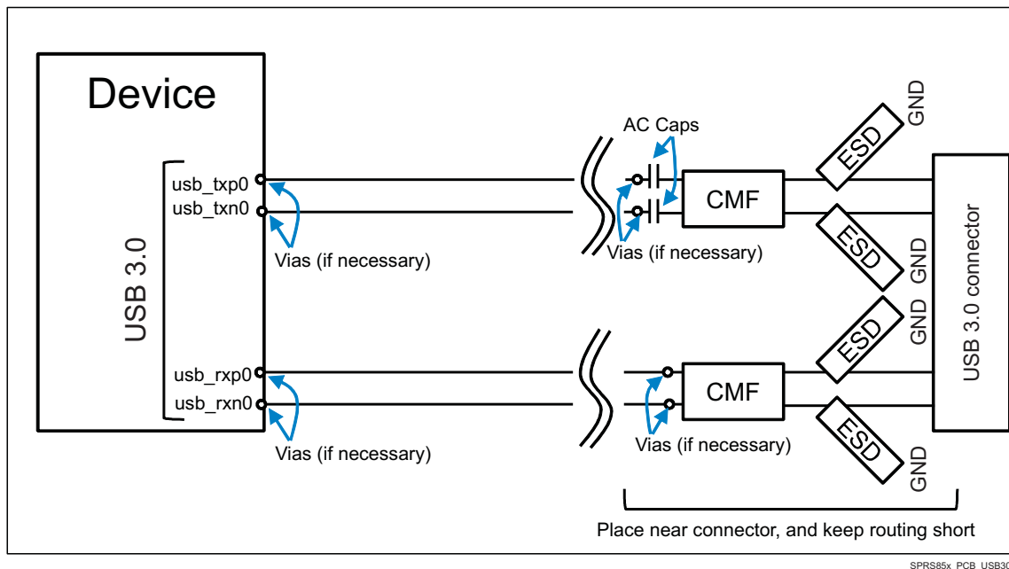
Figure 8-39. USB 3.0 Interface High Level Schematic
