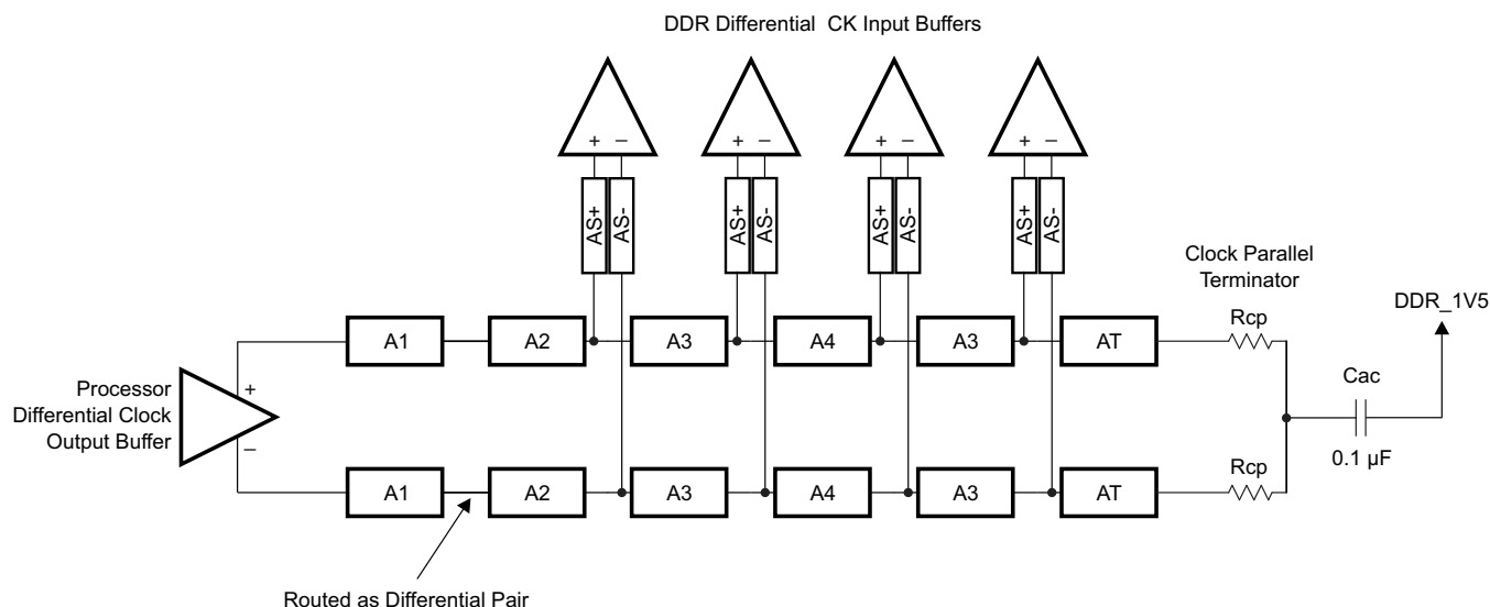
Figure 8-62. CK Topology for Four x8 DDR3 Devices
