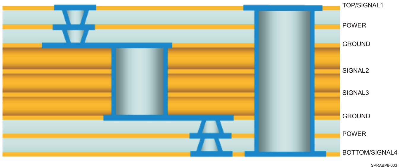
Figure 8-3. Layer PCB With Plated Through Holes (PTH) Vias
