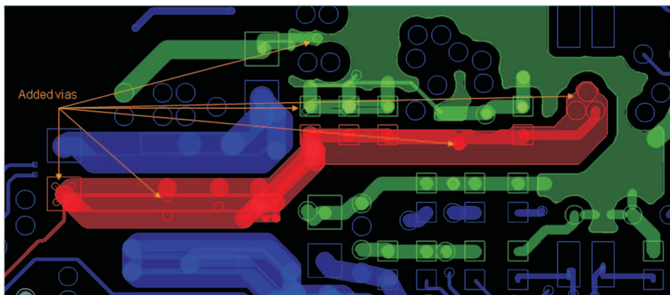
Figure 8-5. Improved Via Assignment for PDN
