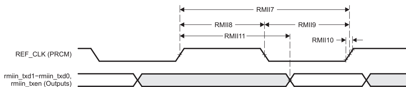
Figure 7-58. GMAC Transmit Interface Timing RMII n Operation
