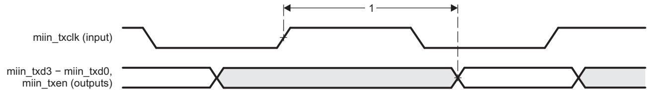
Figure 7-55. GMAC Transmit Interface Timing MII operation
