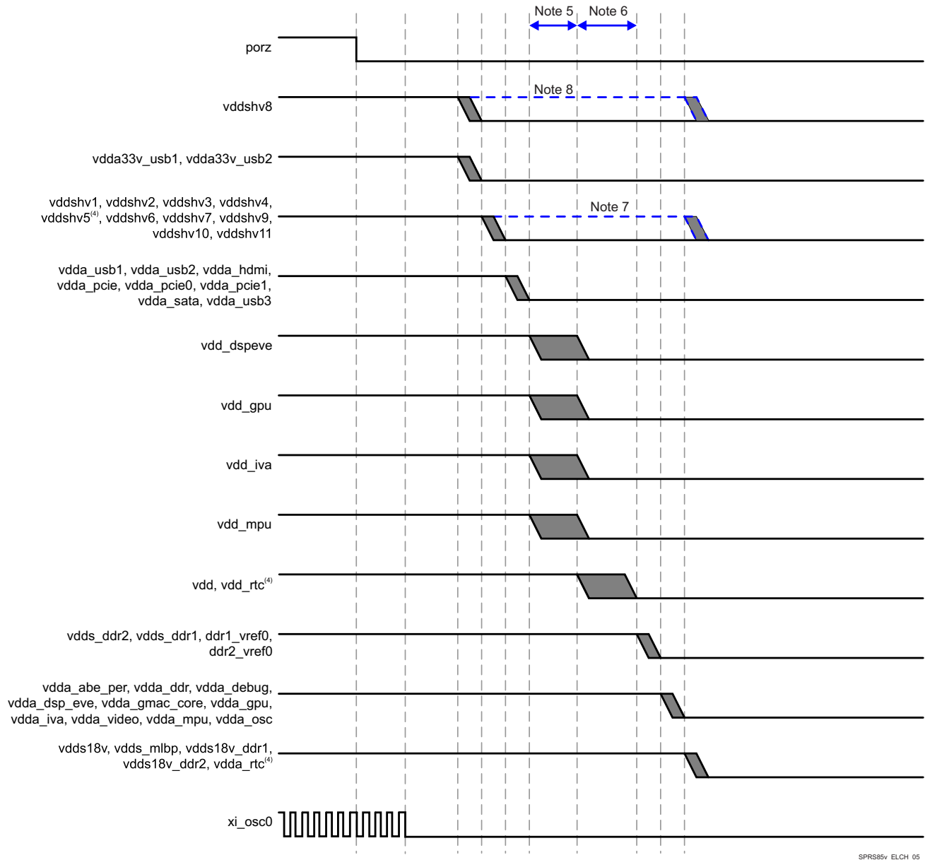
Figure 5-5. Power-Down Sequencing
