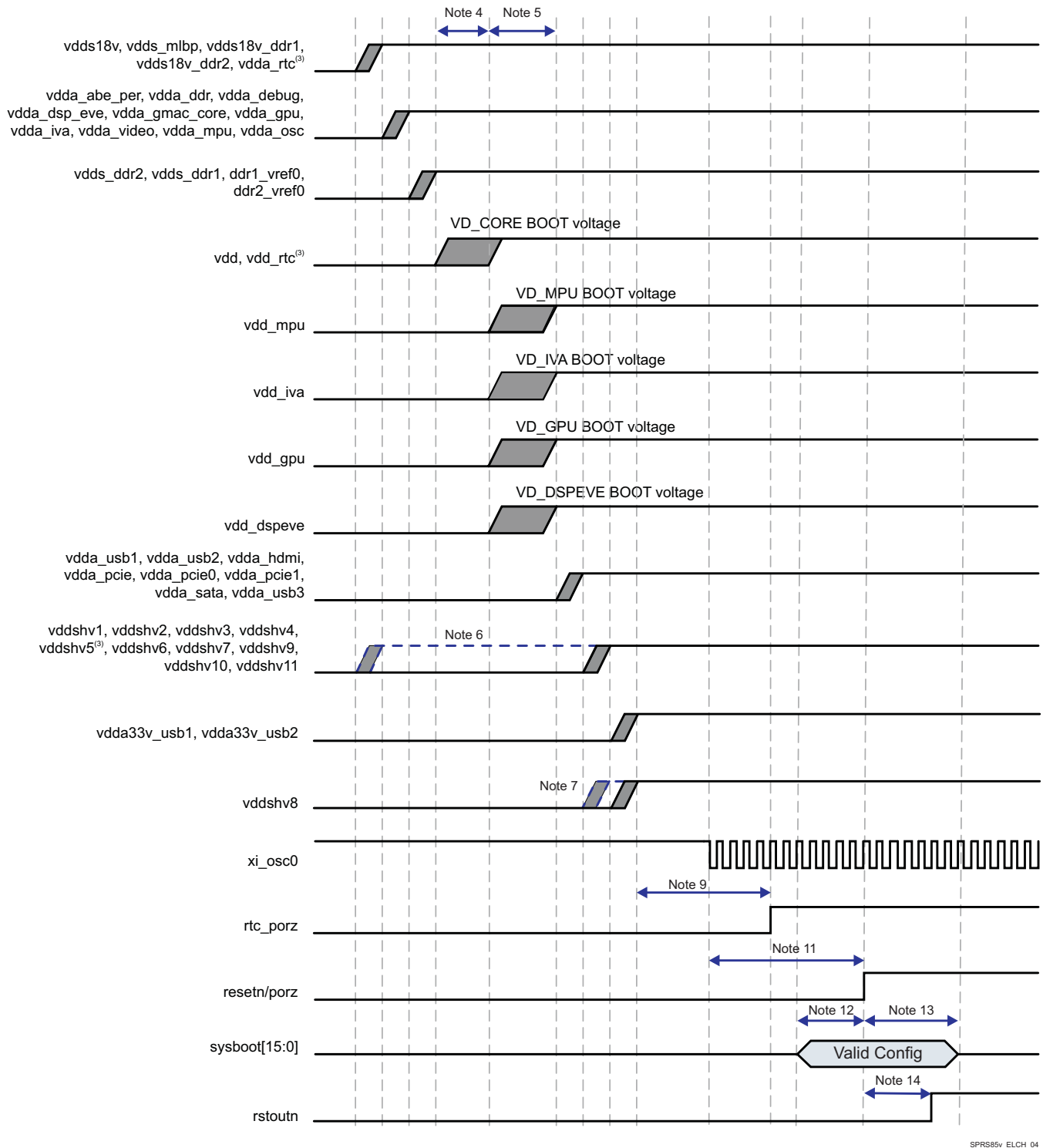
Figure 5-4. Power-Up Sequencing
