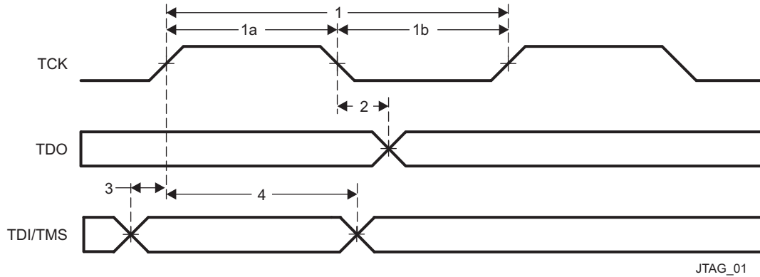
Figure 7-94. JTAG Timing
