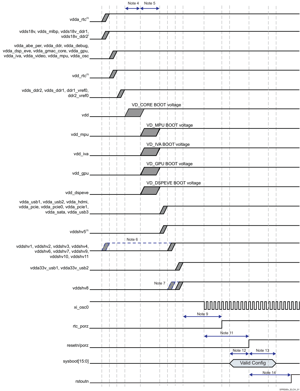
Figure 5-1. Power-Up Sequencing
