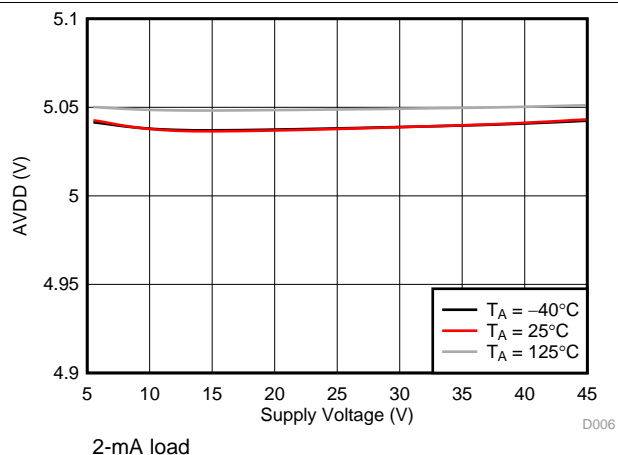
Figure 8. AVDD Regulator
