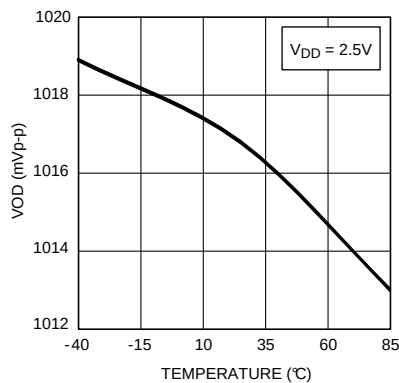
Figure 9. Output Differential Voltage (VOD = 1.0 Vp-p) vs. Temperature
