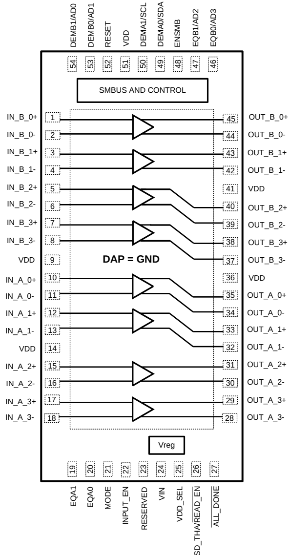
Figure 1. DS100KR800 Pin Diagram 54 lead
