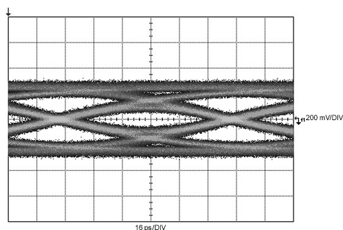
Figure 14. TL1 = 20 inch 4-mil FR4 trace, TL2 = 15 inch 4-mil FR4 trace, DS100KR800 settings: EQ[1:0] = R, R = 15'h, DEM[1:0] = float, float
