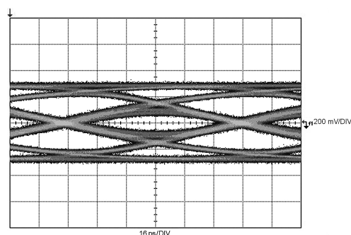
Figure 15. TL1 = 30 inch 4-mil FR4 trace, TL2 = 15 inch 4-mil FR4 trace, DS100KR800 settings: EQ[1:0] = float, R = 1F'h, DEM[1:0] = float, float
