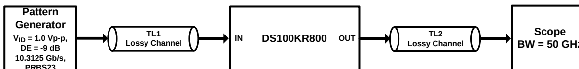
Figure 13. Test Setup Connections Diagram
