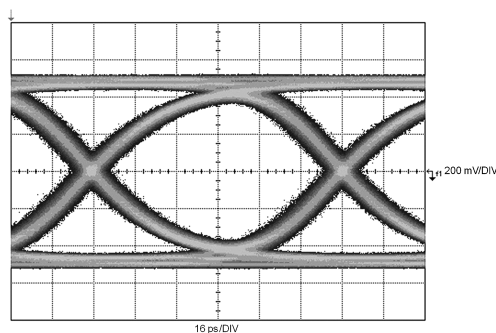
Figure 11. TL = 20 inch 4-mil FR4 trace, DS100KR800 settings: EQ[1:0] = R, R = 15'h, DEM[1:0] = float, float
