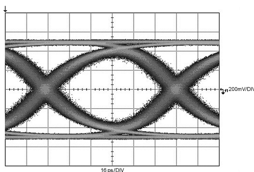
Figure 12. TL = 30 inch 4-mil FR4 trace, DS100KR800 settings: EQ[1:0] = float, R = 1F'h, DEM[1:0] = float, float
