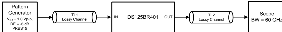
Figure 22. Test Setup Connections Diagram
