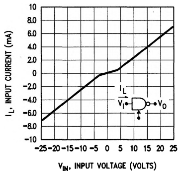
FIGURE 2. Input Current
