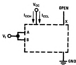
FIGURE 4. I_{CCH} for AND and NAND Circuits
