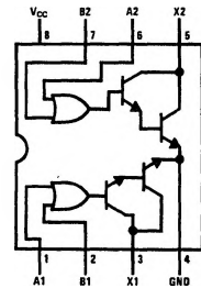
Top View Order Number DS1634J-8 or DS3634N
