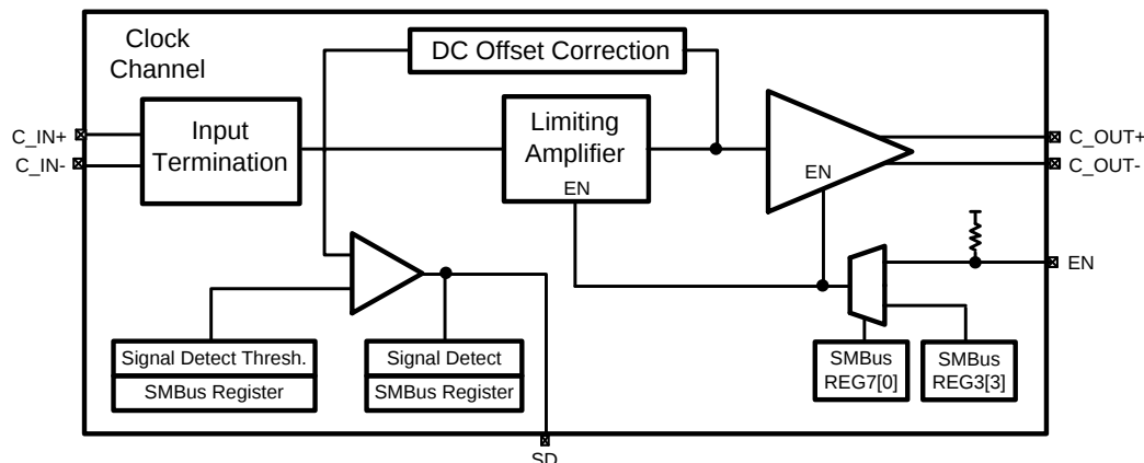
Figure 4. DS16EV5110A Clock Channel
