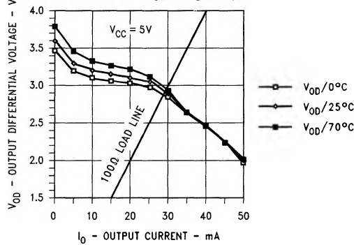
DS26LS31CN V_{OD} vs I_O vs T_A
