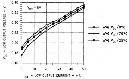
DS26LS31CN V_{OL} vs I_{OL} vs T_A
