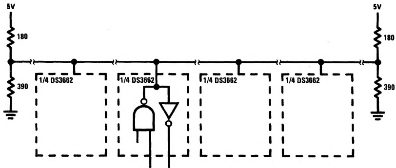
120 \Omega Unified Data Bus
