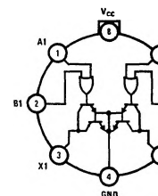
Top View (Pin 4 is electrically connected to the case.) Order Number DS1634H
