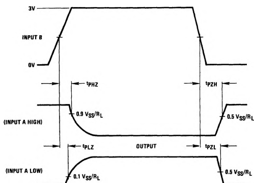
FIGURE 4. TRI-STATE Delays
