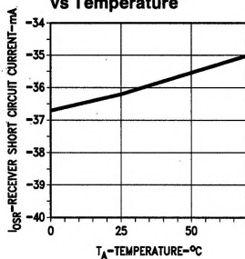
Receiver Short Circuit Current vs Temperature
