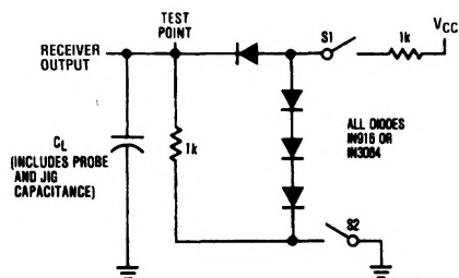
FIGURE 1. Receiver Propagation Delay Test Circuit
