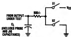
FIGURE 4. Driver Propagation Delay Test Circuits
