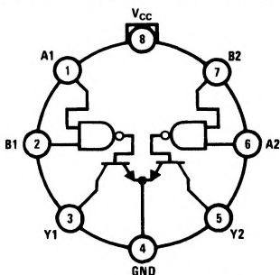
TL/F/5824-6
