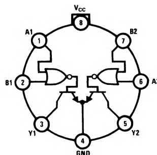
TL/F/5824-8
