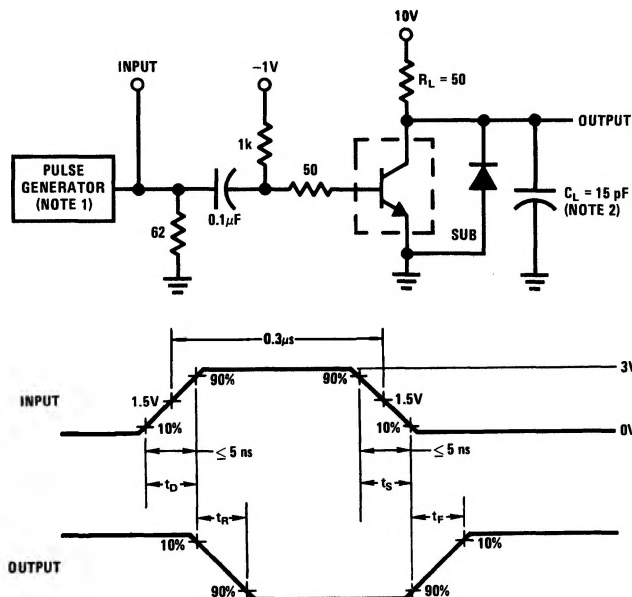
FIGURE 12. Propagation Delay Times, Each Gate
