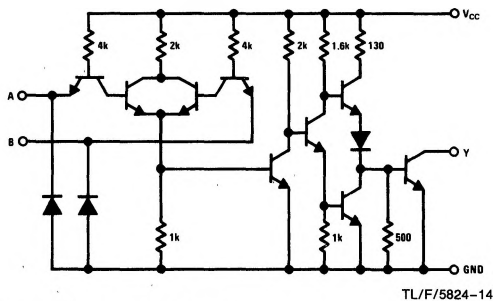
DS55454/DS75454
