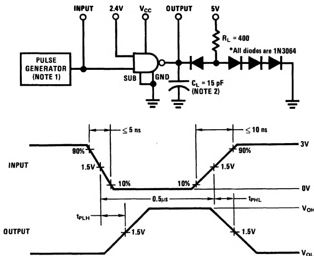
FIGURE 12. Propagation Delay Times, Each Gate
