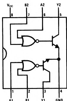
TL/F/5824-4
