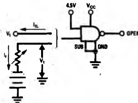
FIGURE 3. V_I , I_{IL}
