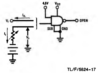
Each input is tested separately. FIGURE 3. V_I , I_L
