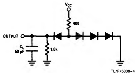
FIGURE 2. Receiver Output Load
