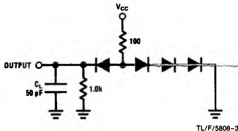
FIGURE 1. Driver Output Load
