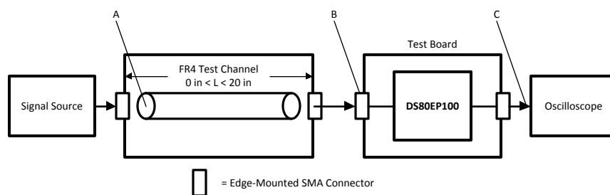
Figure 2. Transient Test Setup Diagram
