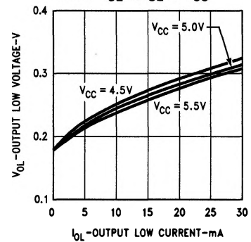
Driver V_{OL} vs I_{OL} vs V_{CC}
