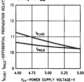
Driver Differential Propagation Delay vs V_{CC}
