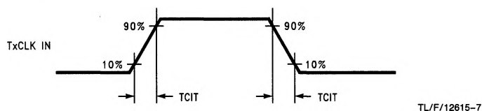
FIGURE 5. DS90CF563 (Transmitter) Input Clock Transition Time
