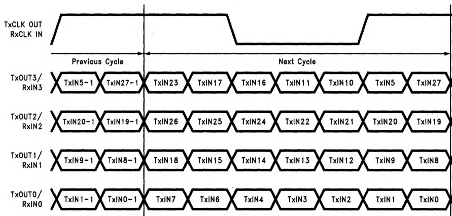
FIGURE 14. Parallel TTL Data Inputs Mapped to LVDS Outputs (DS90CF583)
