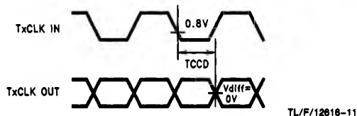
FIGURE 9. DS90CF583 (Transmitter) Clock In to Clock Out Delay
