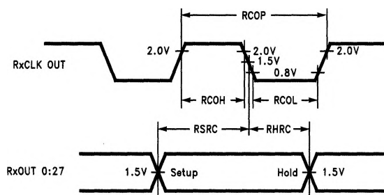
FIGURE 8. DS90CF584 (Receiver) Setup/Hold and High/Low Times
