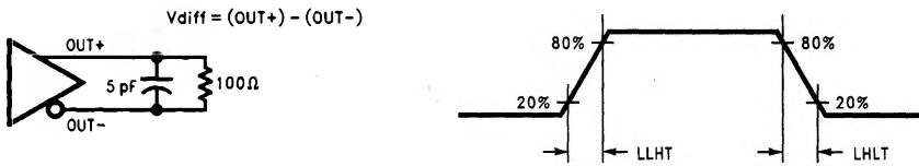
FIGURE 3. DS90CF583 (Transmitter) LVDS Output Load and Transition Times
