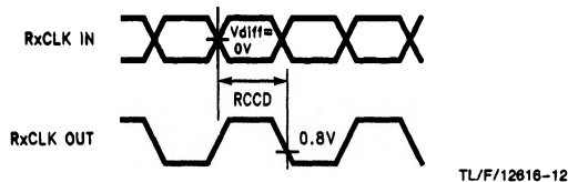
FIGURE 10. DS90CF584 (Receiver) Clock In to Clock Out Delay
