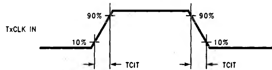
FIGURE 5. DS90CF583 (Transmitter) Input Clock Transition Time
