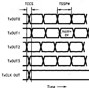
FIGURE 6. DS90CF583 (Transmitter) Channel-to-Channel Skew and Pulse Width
