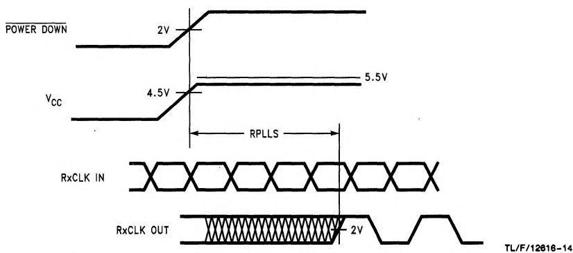
FIGURE 12. DS90CF584 (Receiver) Phase Lock Loop Set Time
