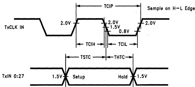
FIGURE 7. DS90CF583 (Transmitter) Setup/Hold and High/Low Times
