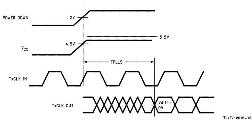
FIGURE 11. DS90CF583 (Transmitter) Phase Lock Loop Set Time
