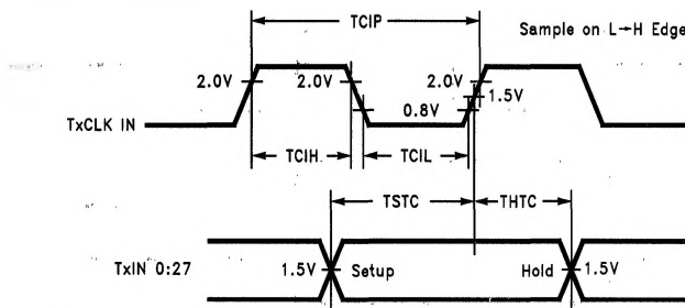
FIGURE 6. DS90CR281 (Transmitter) Setup/Hold and High/Low Times
