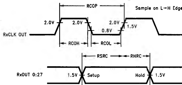
FIGURE 7. (Receiver) DS90CR282 Setup/Hold and High/Low Times
