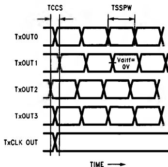
FIGURE 5. DS90CR281 (Transmitter) Channel-to-Channel Skew and Pulse Width
