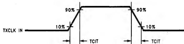
FIGURE 4. DS90CR281 (Transmitter) Input Clock Transition Time
