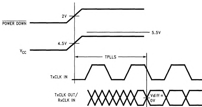
FIGURE 10. DS90CR281 (Transmitter) Phase Lock Loop Set Time
