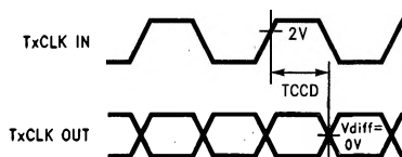
FIGURE 8. DS90CR281 (Transmitter) Clock In to Clock Out Delay
