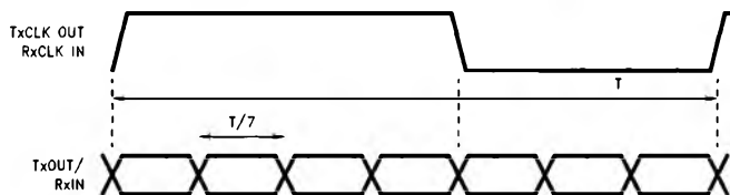
FIGURE 12. Seven Bits of LVDS in One Clock Cycle
