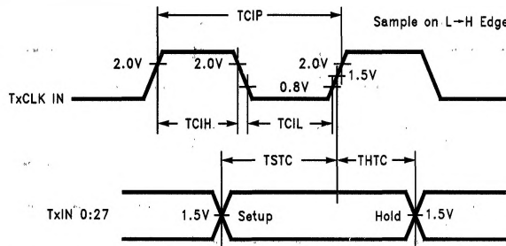
FIGURE 6. DS90CR281 (Transmitter) Setup/Hold and High/Low Times
