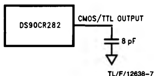
FIGURE 3. DS90CR282 (Receiver) CMOS/TTL Output Load and Transition Timing
