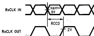
FIGURE 9. DS90CR282 (Receiver) Clock In to Clock Out Delay
