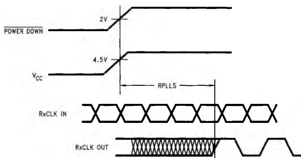
FIGURE 11. DS90CR282 (Receiver) Phase Lock Loop Set Time
