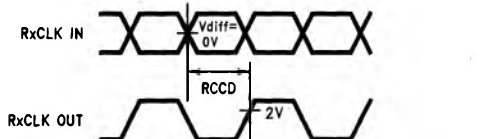
FIGURE 10. DS90CR562 (Receiver) Clock In to Clock Out Delay
