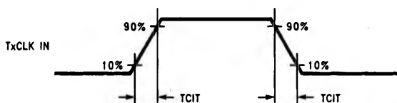
FIGURE 5. DS90CR583 (Transmitter) Input Clock Transition Time
