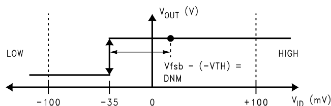
Figure 6. VTC of the DS90LV048A LVDS Receiver
