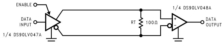
Figure 5. Point-to-Point Application
