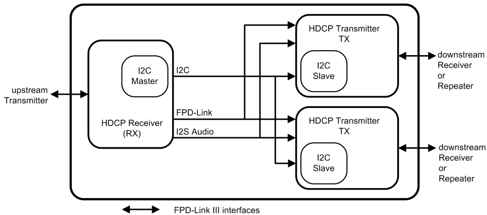
FIGURE 18. HDCP 1:2 Repeater Configuration
