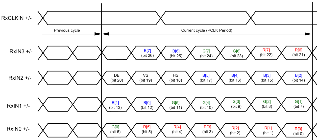
FIGURE 13. FPD-Link Mapping: MSBs on RxIN3 (MAPSEL=H)
