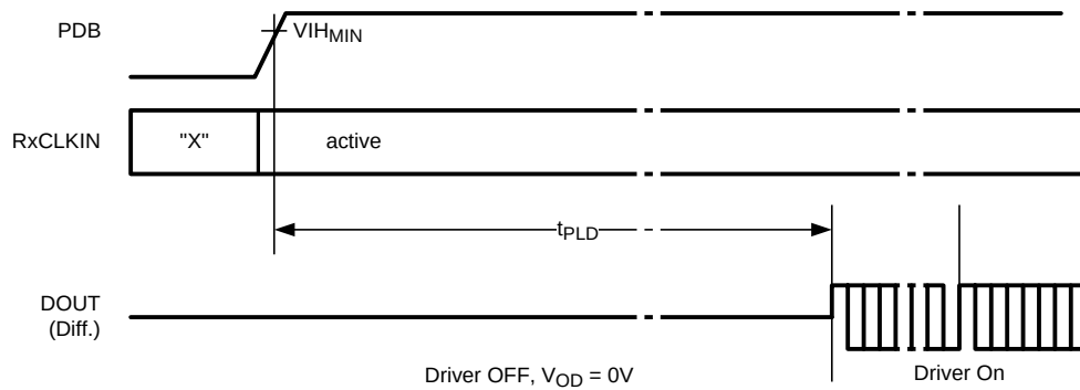
Figure 10. DS92LV0421 Lock Time
