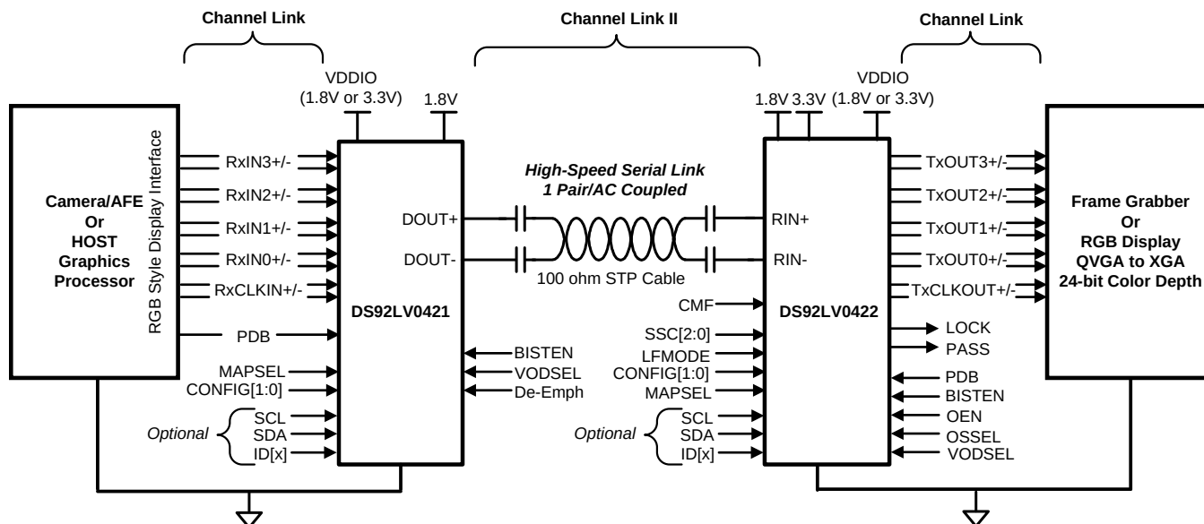
Figure 1. Application Diagram
