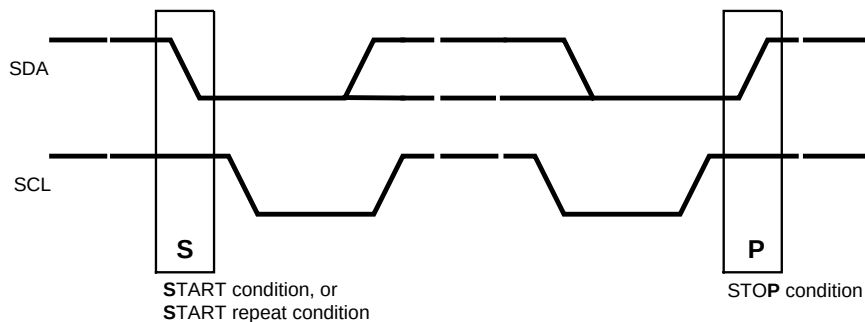
Figure 31. START and STOP Conditions
