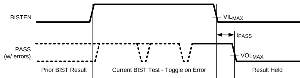
Figure 20. BIST PASS Waveform
