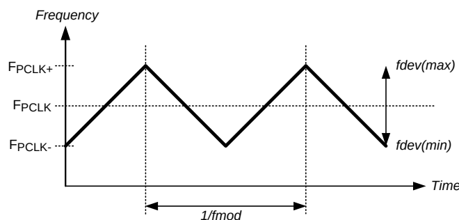
Figure 27. SSCG Waveform
